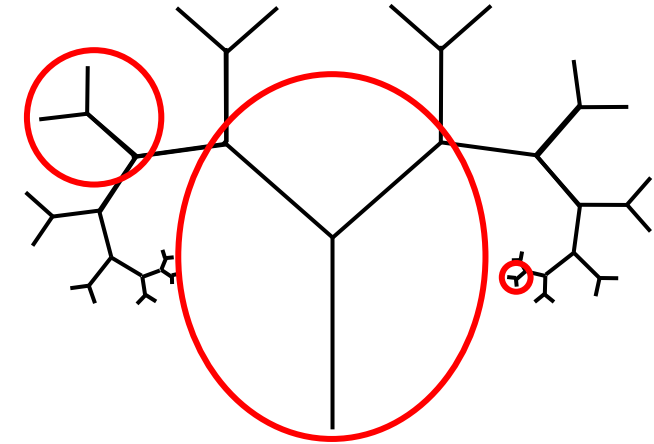
Exact self-similar Fractal
